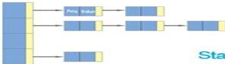
HashMap
