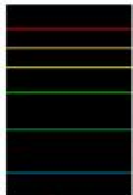
Line Spectrum
