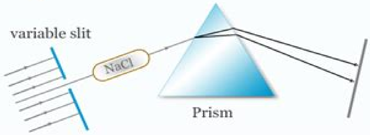
ABSORPTION SPECTRUM
