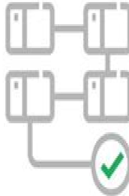
Software Component
