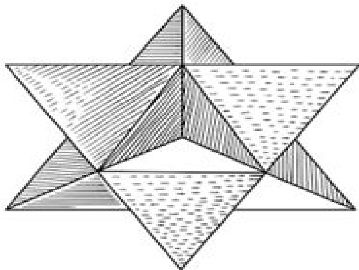
• STELLATE OCTAHEDRON •
