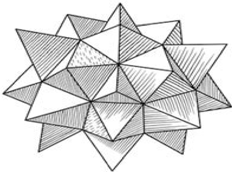
• STAR ICOSAHEDRON •
