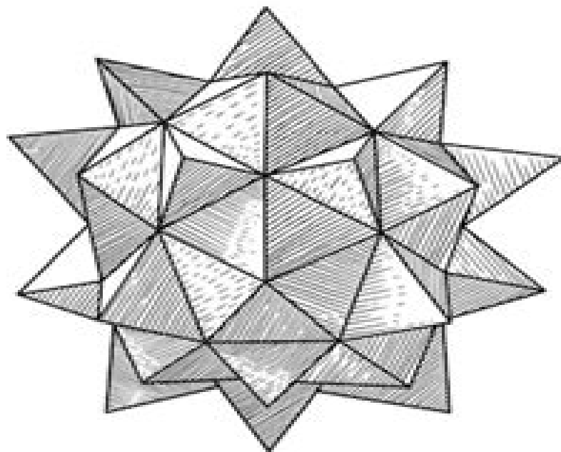
• STAR DODECAHEDRON •
