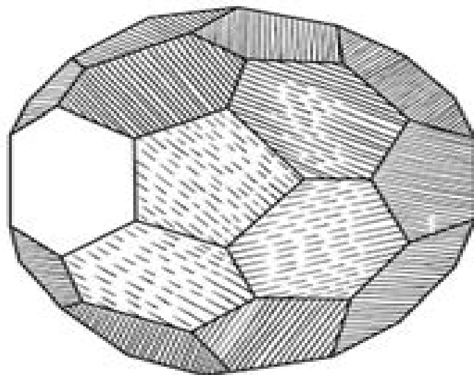
• ICOSAHEDRON TRUNCATED •
