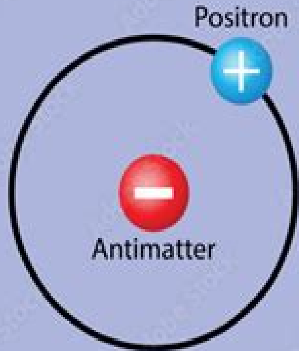
Antihydrogen
