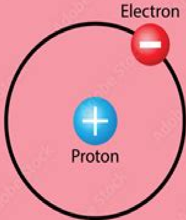
Hydrogen
