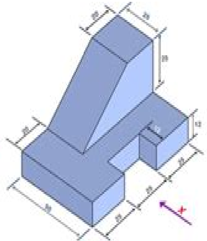
Isometric View
