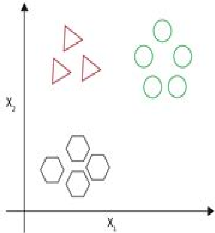
Multi-class Classification
