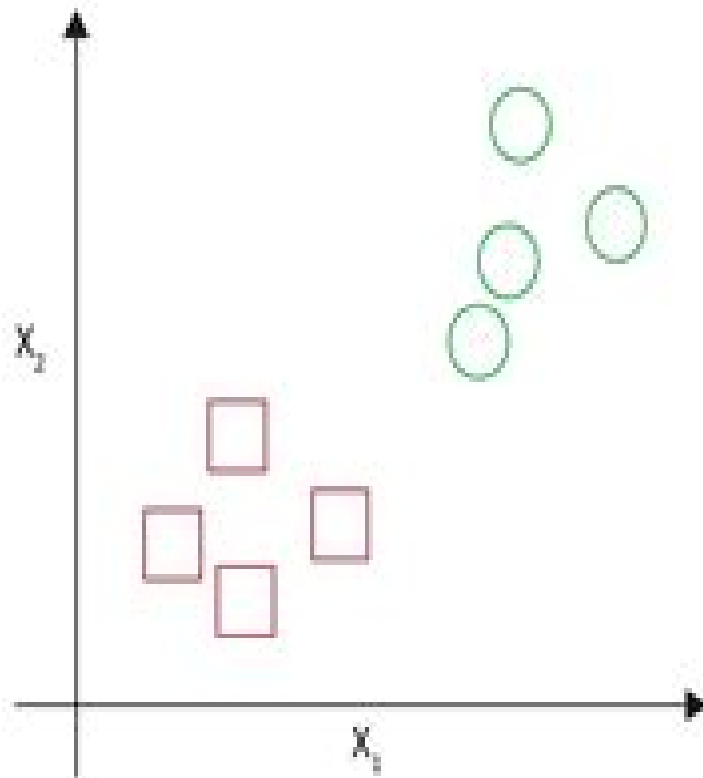
Binary Classification
