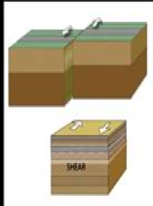
Strike-slip fault
