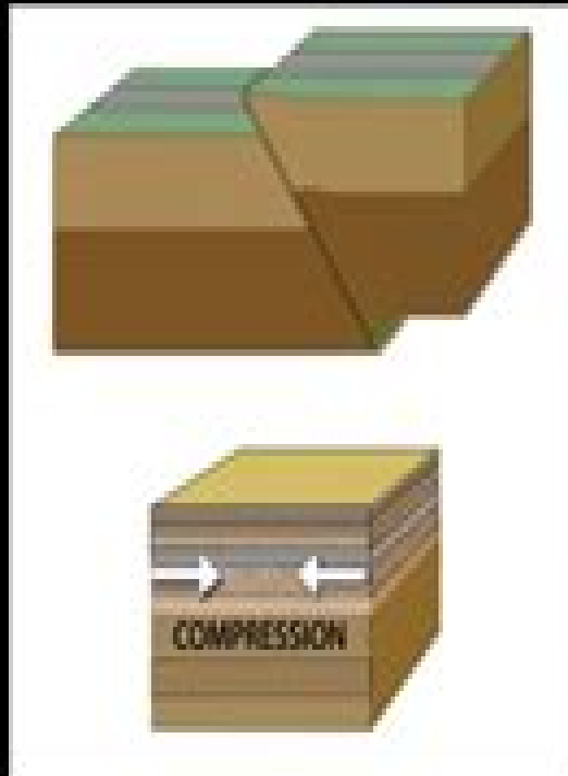
Reverse fault
