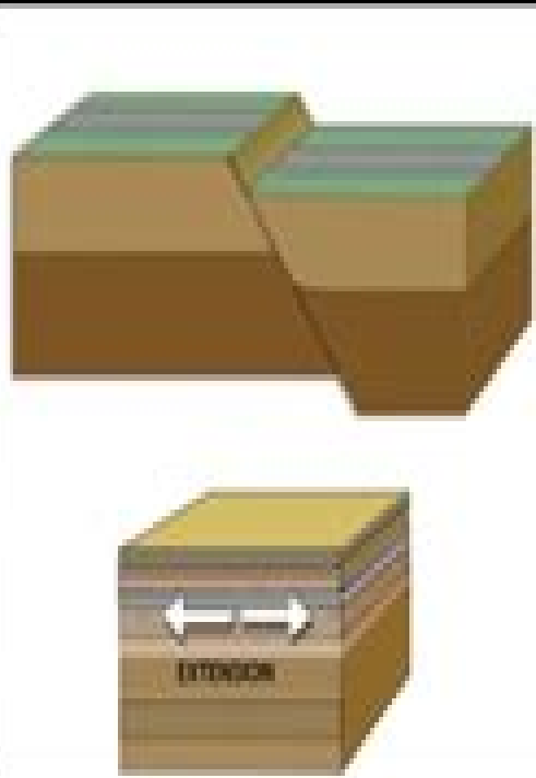
Normal fault
